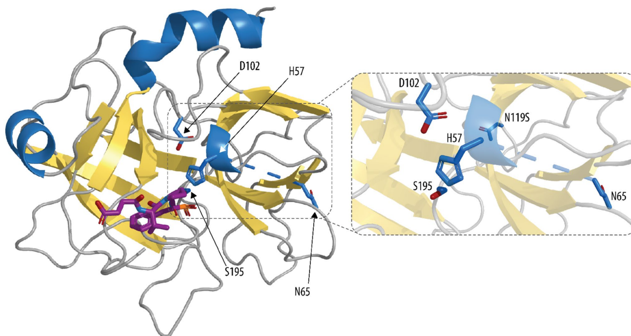
Fig. 1 Three-dimensional structure of human CatG (ribbon plot). The catalytic triad of CatG is indicated by H 57 , D 102 , and S 195 which is located between the two asymmetric barrels and depicted in yellow. The C-terminal \alpha -helix is shown on top and presented in blue. The
